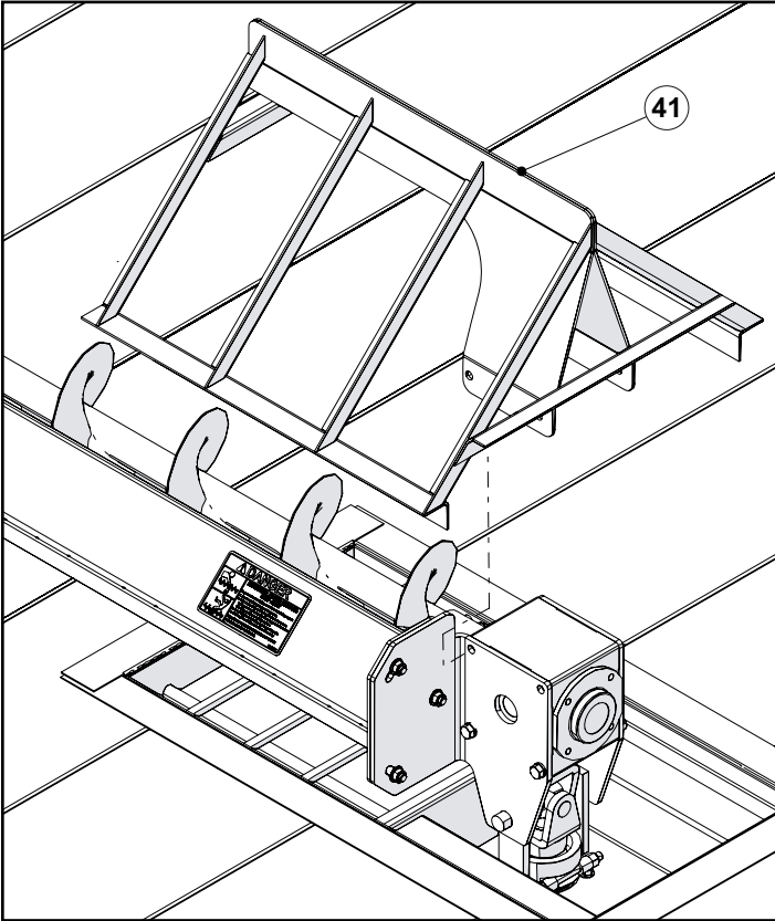
Fig. # 3-2 Clump Buster Installation
