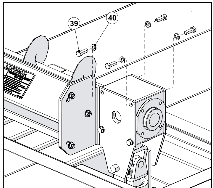
Fig. # 3-1 Clump Buster Installation
