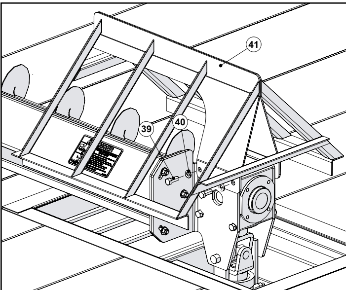
Fig. # 3-3 Clump Buster Installation
