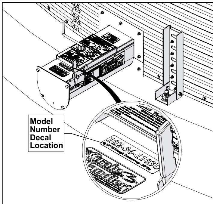
Fig. # 1-4 Locating Model Number Decal (Power Sweep & U-Trough)
