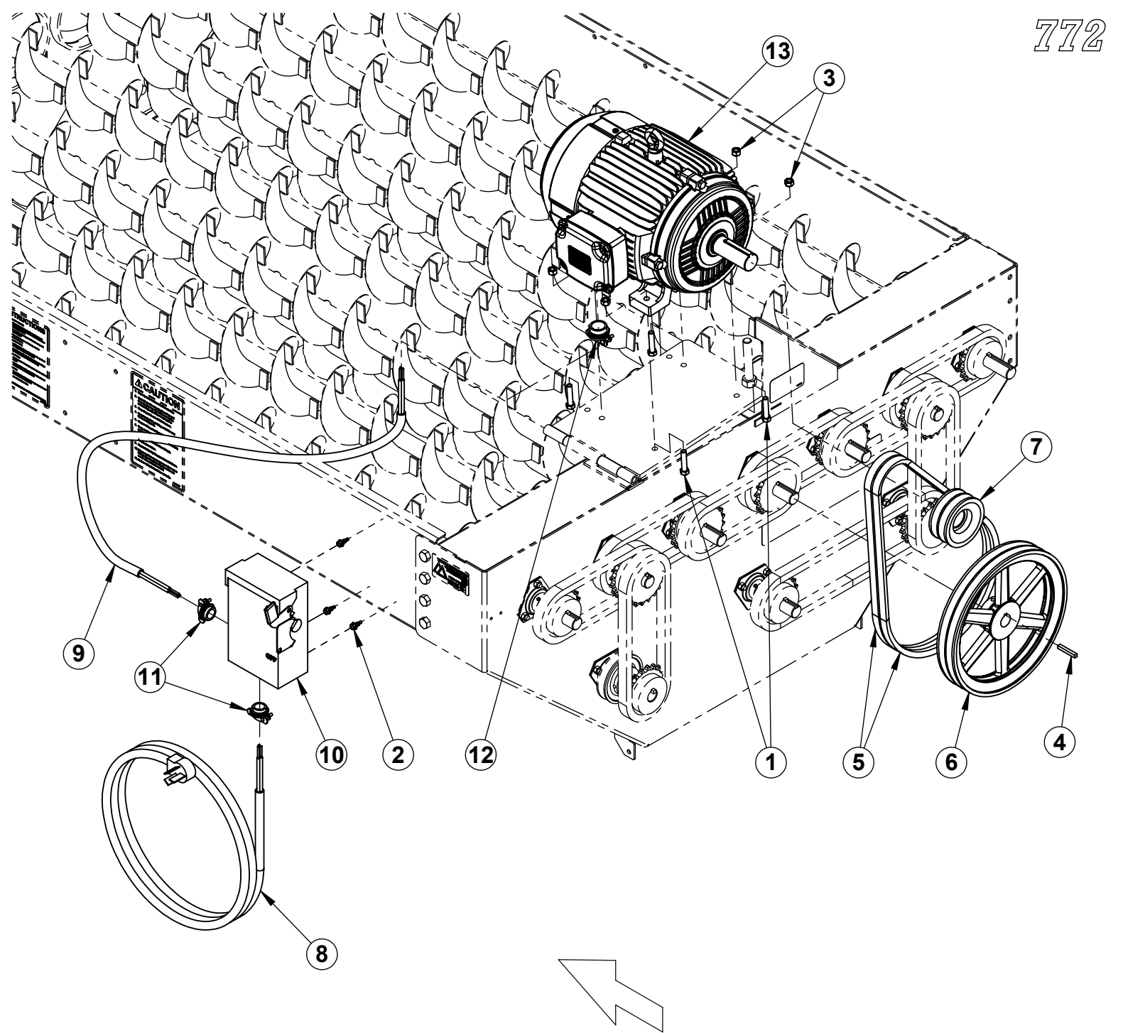
45-1-00011 ELECTRIC DRIVE KIT (7.5 HP, 220V, 1-PHASE) - 772
