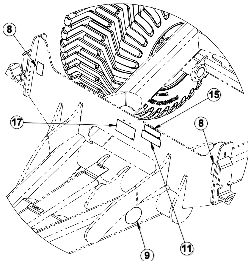
DETAIL A
