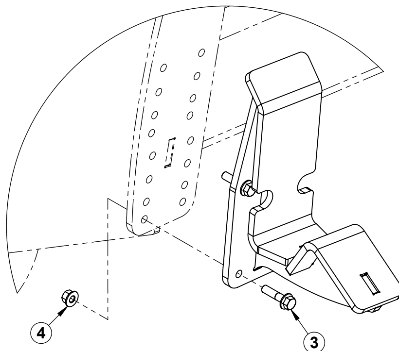
DETAIL A
