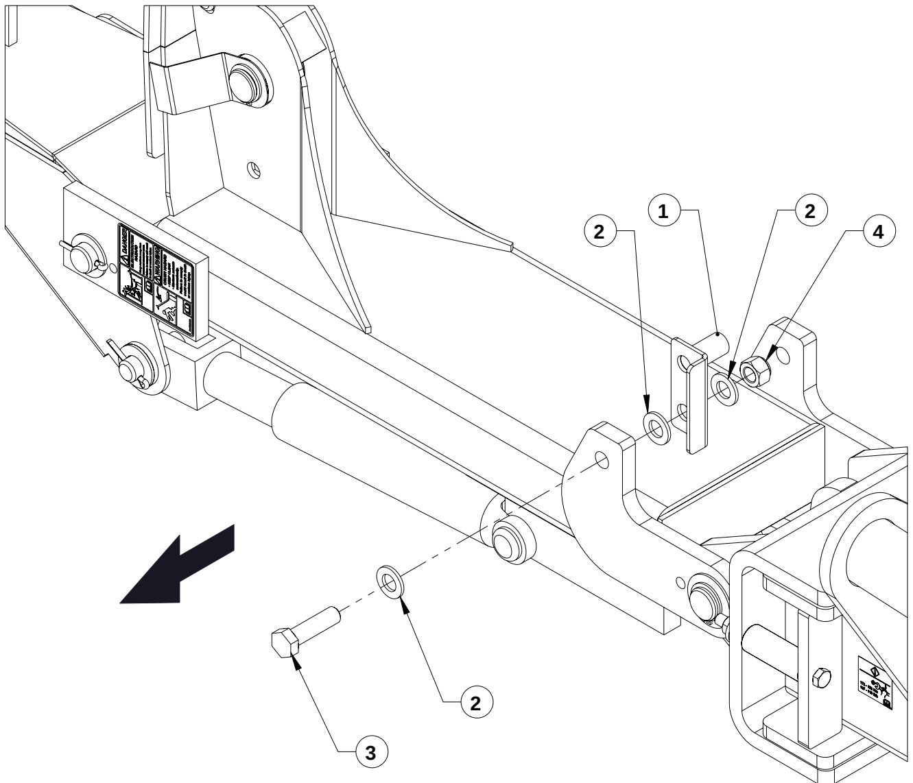
Right Wing Marker Stop Detail
