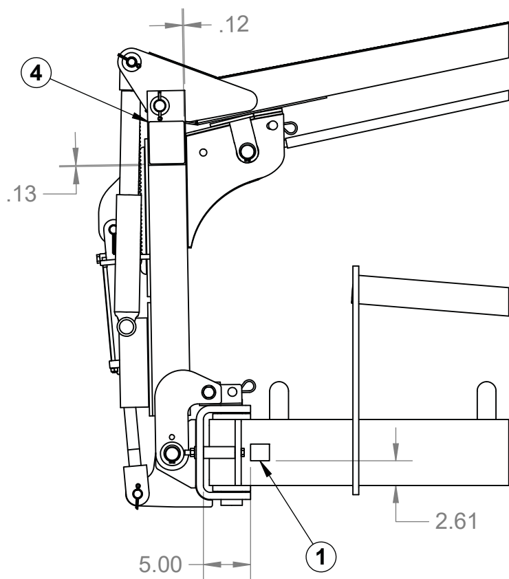
Front View Right Wing Row Marker Decal Locations (Repeat For Left Wing)
