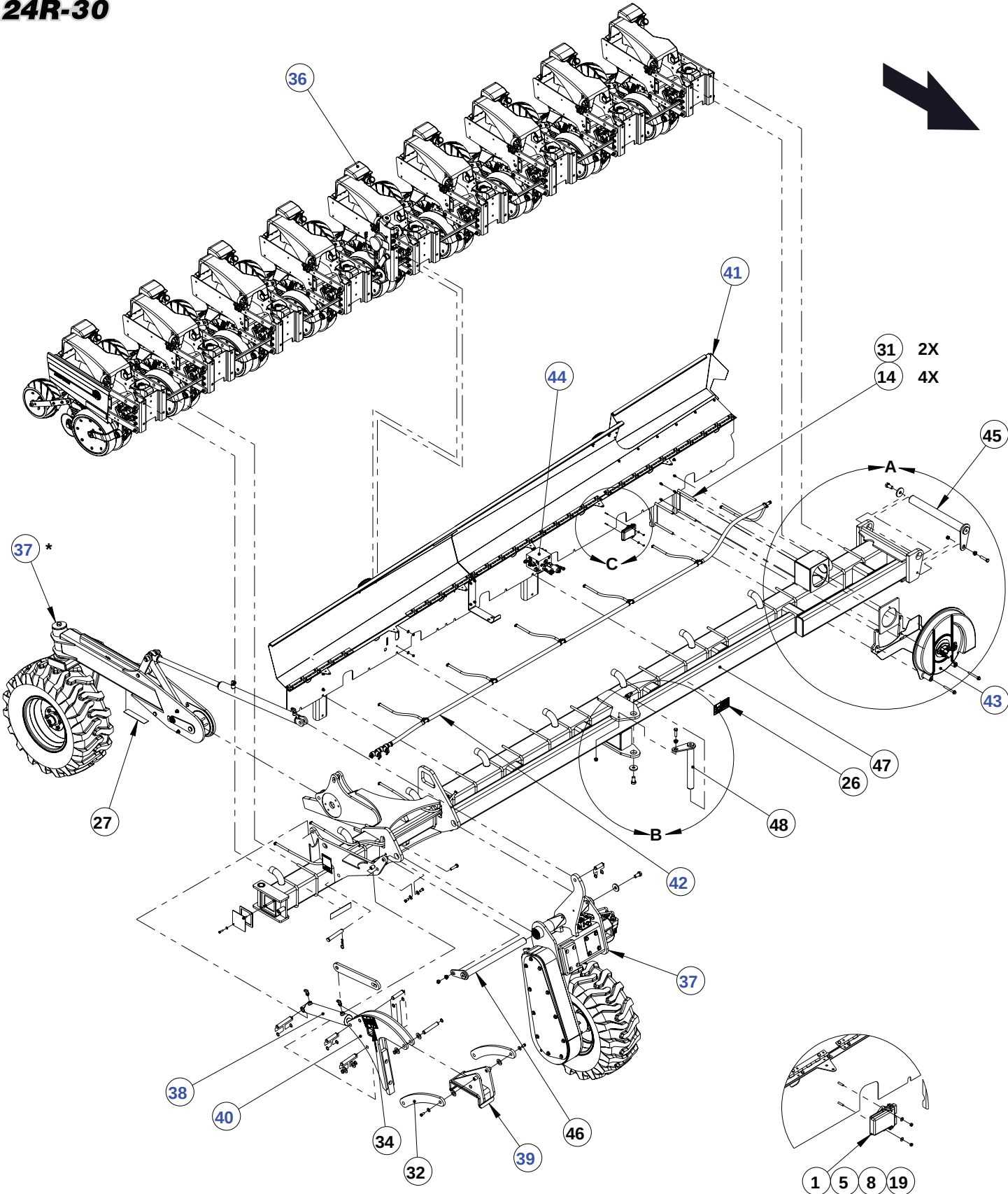
DETAIL C SCALE 1 : 20
