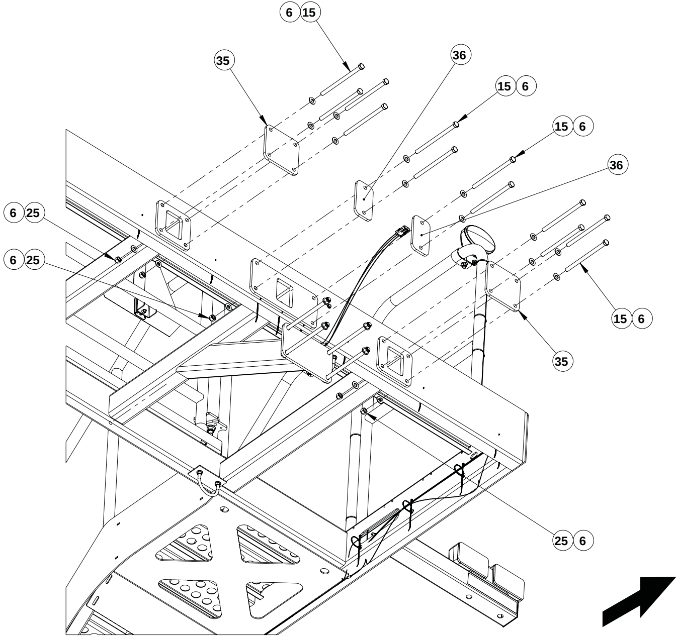
Platform Mounting
