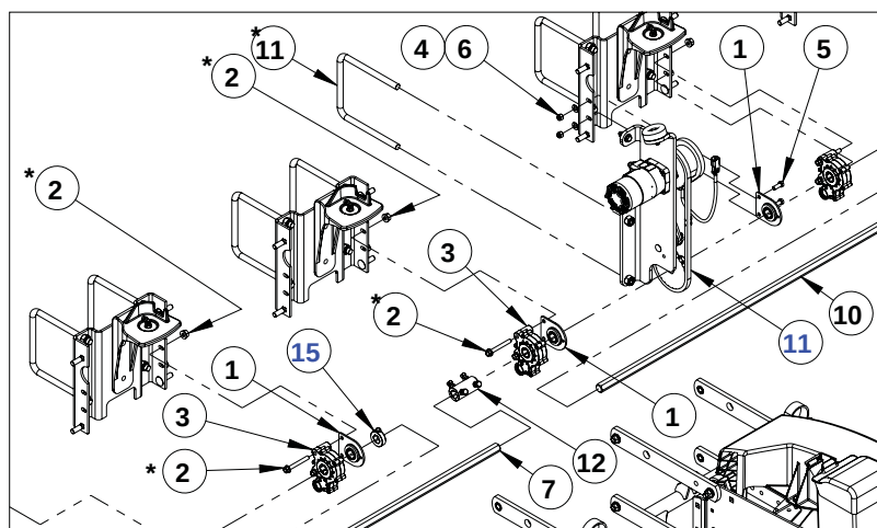
DETAIL C SCALE 1 : 20
