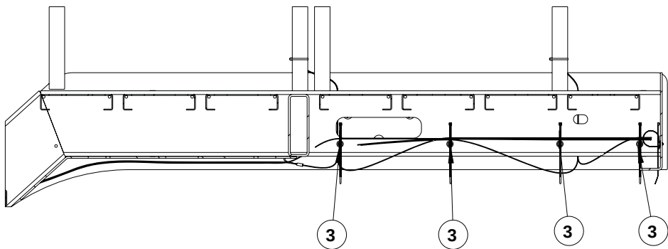
Cable Tie Mount Locations (Left Side, Inside) SECTION C-C SCALE 1 : 12
