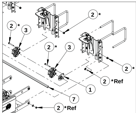
DETAIL D SCALE 1 : 20
