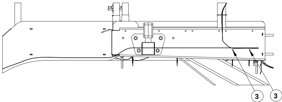
Cable Tie Mount Locations (Right Side)
