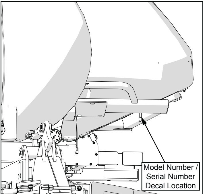
Fig. # 1-5 Model / Serial Number Decal Location On Bulk Fill Assembly
