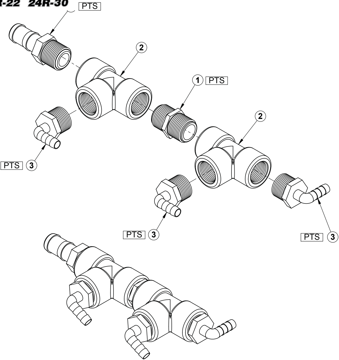
Assembled View Left Hand Application
