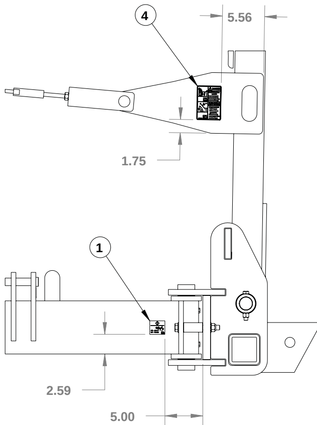
Front View Left Wing Row Marker Decal Locations (Repeat For Right Wing)
