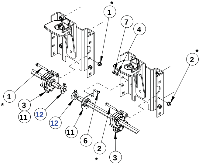
DETAIL C SCALE 1 : 12
