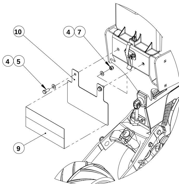
DETAIL A SCALE 1 : 8
