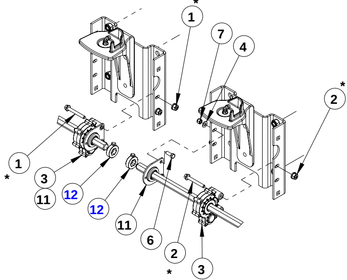
DETAIL C
