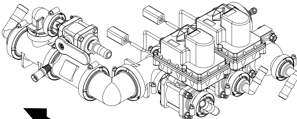
Assembled View
