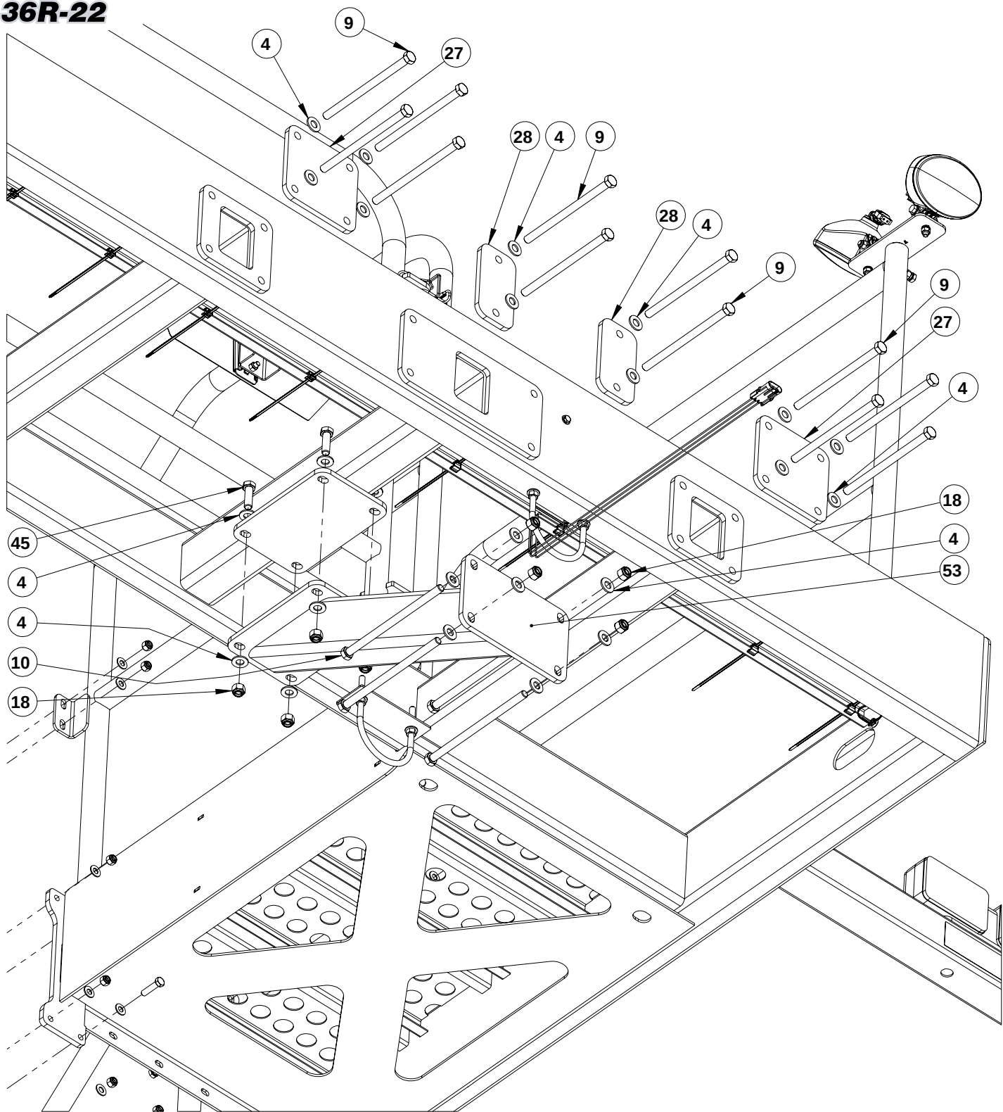
Platform Mounting
