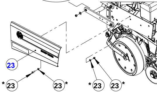
DETAIL D SCALE 1 : 20
