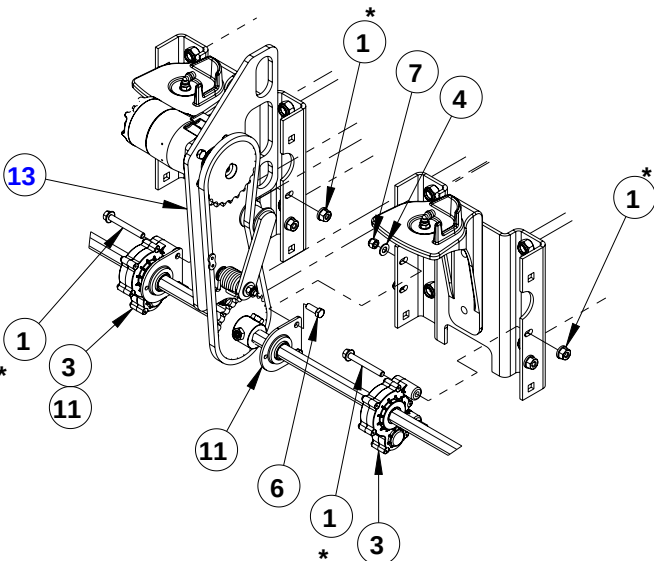
DETAIL B
