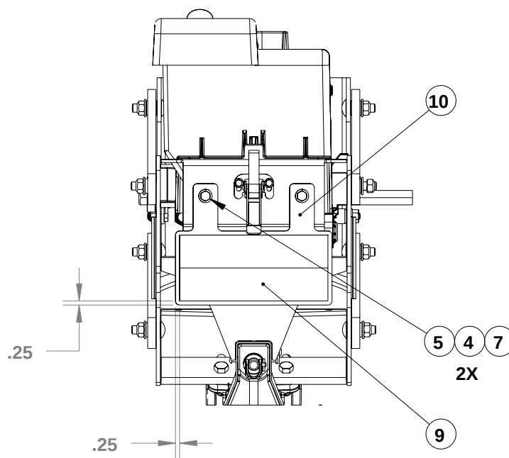
DECAL PLACEMENT
