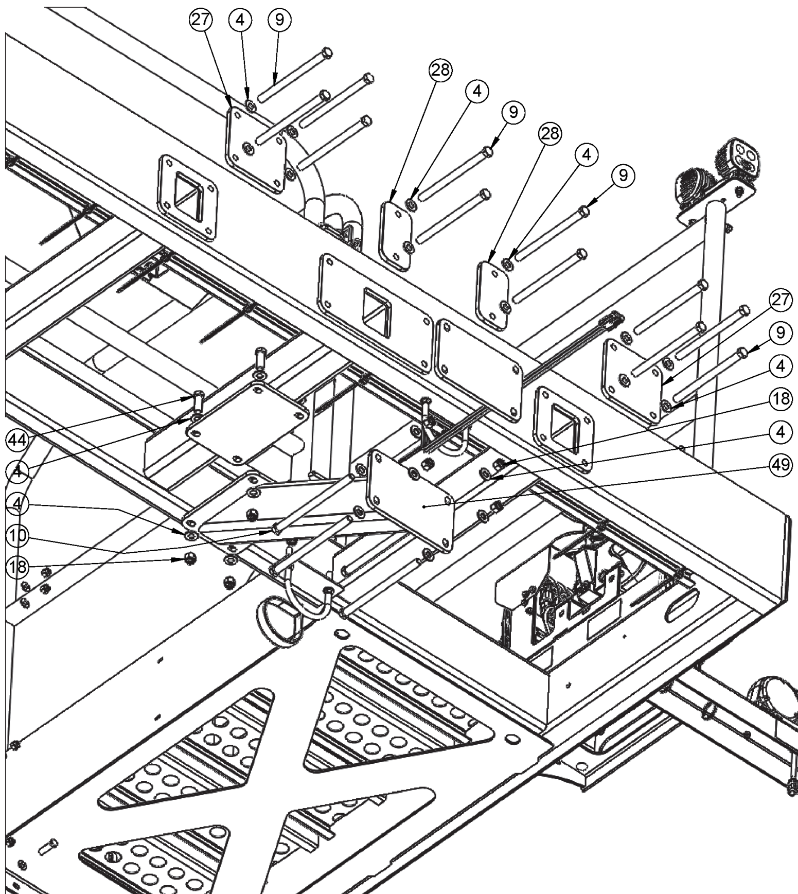
Platform Mounting
