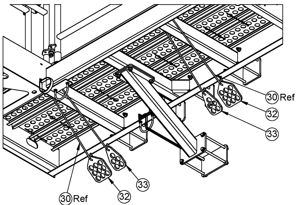
J-Hangers
