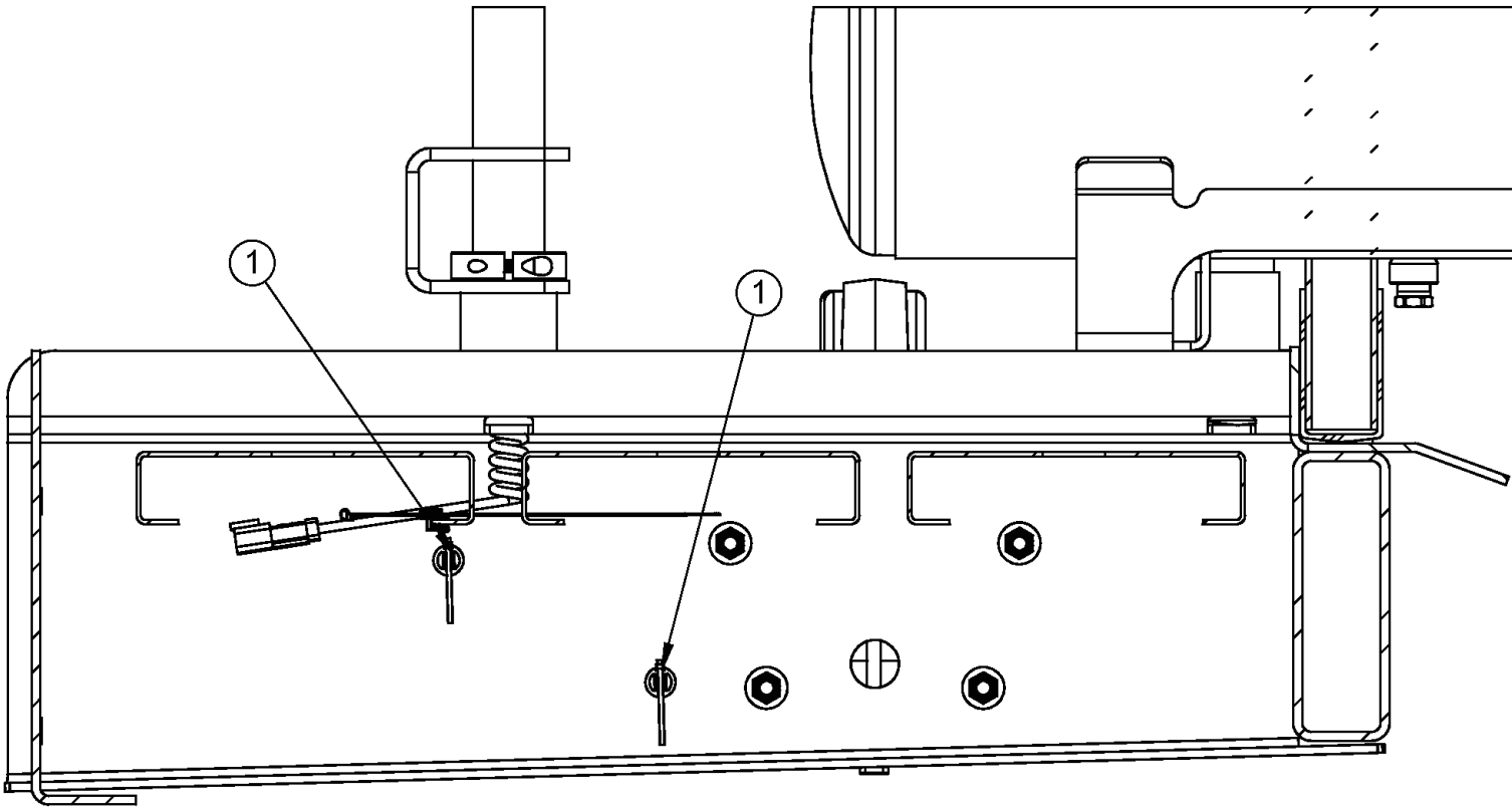
Cable Tie Mount Locations (Right Side, Looking Outward)
