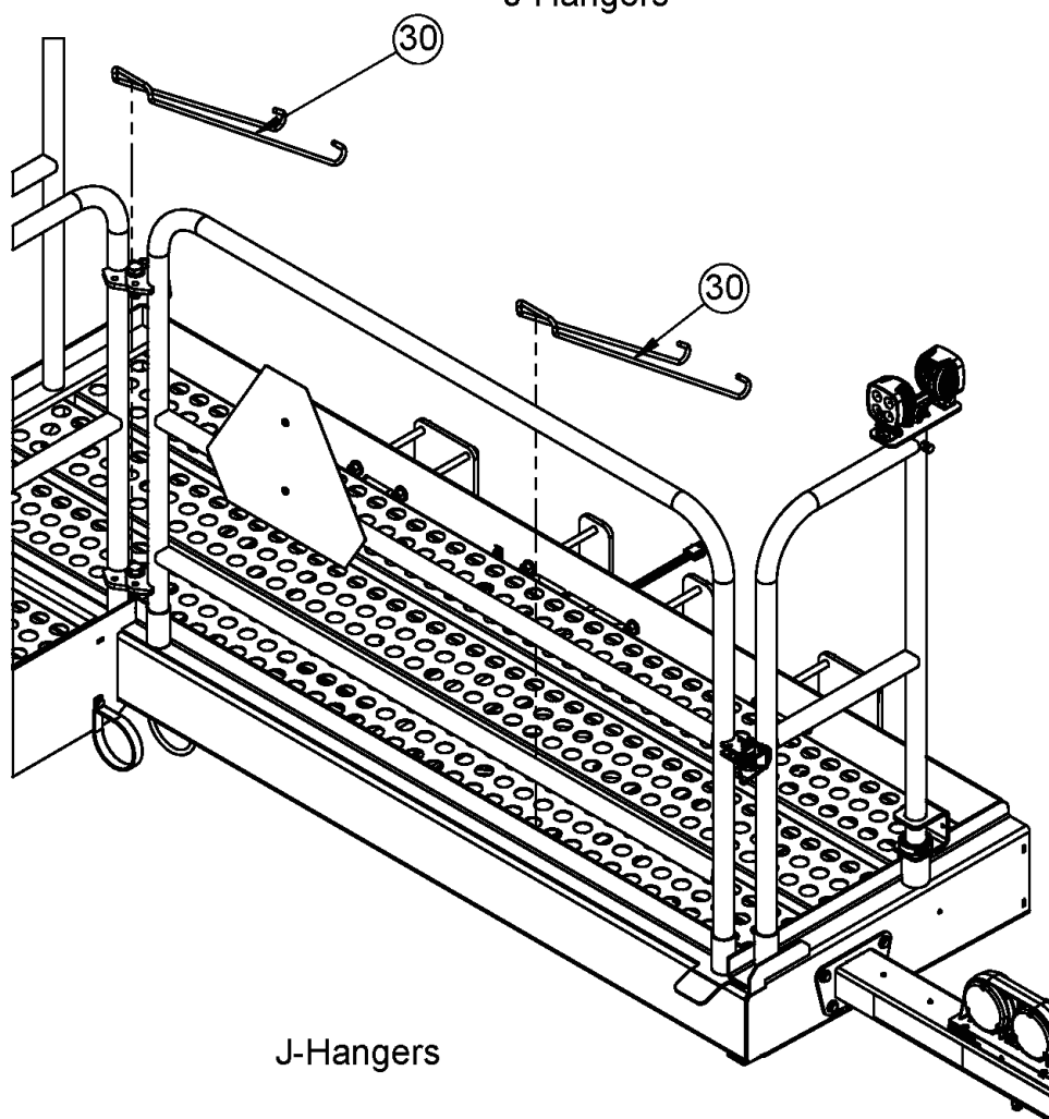
J-Hangers
