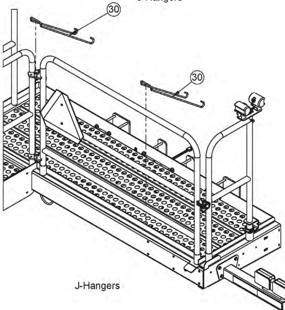
J-Hangers
