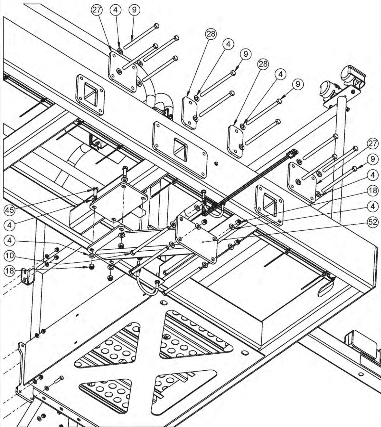
Platform Mounting
