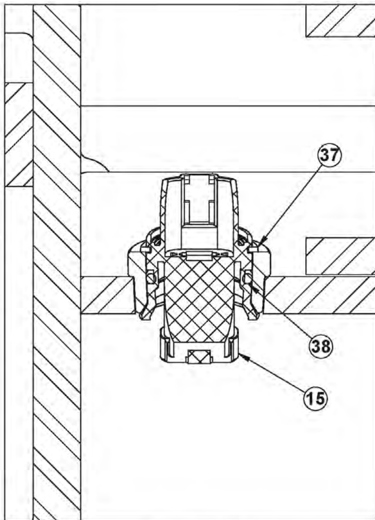
Assembled View
