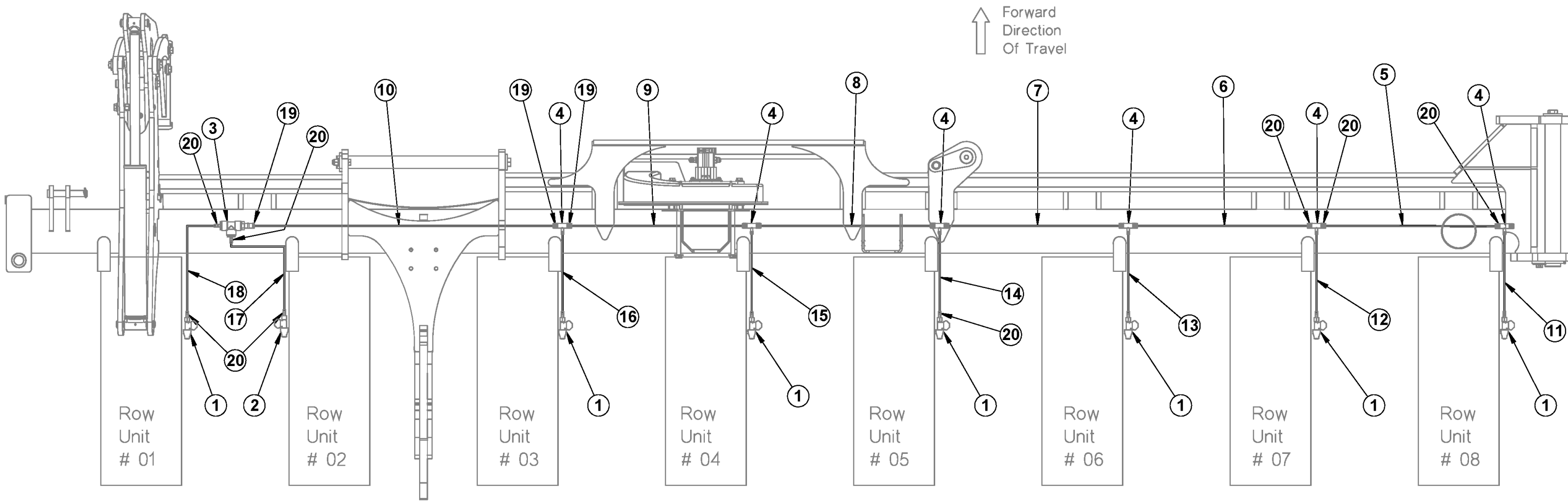
24R-30 Fertilizer Schematic (LH Wing)
