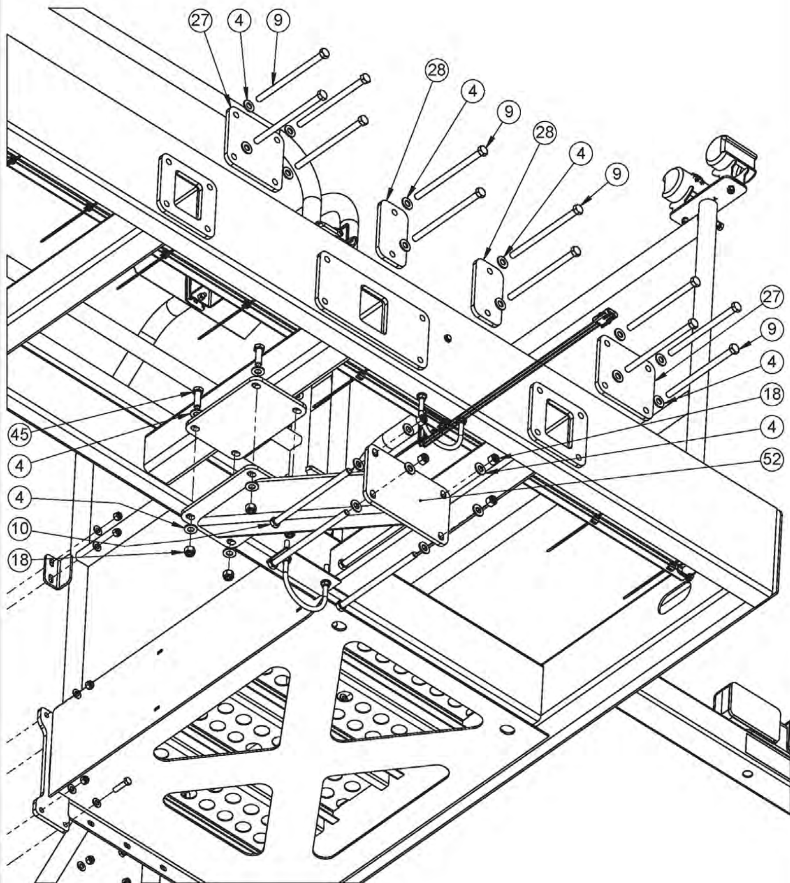
Platform Mounting
