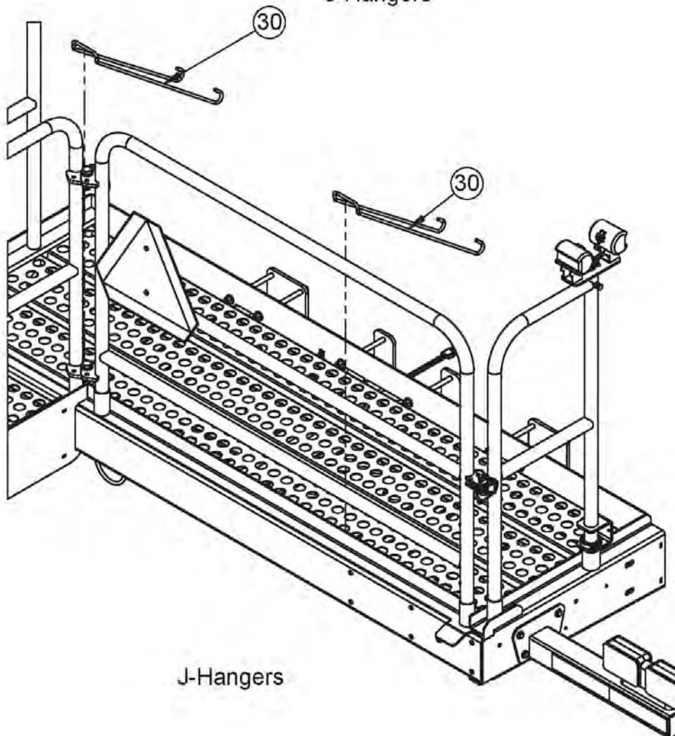
J-Hangers
