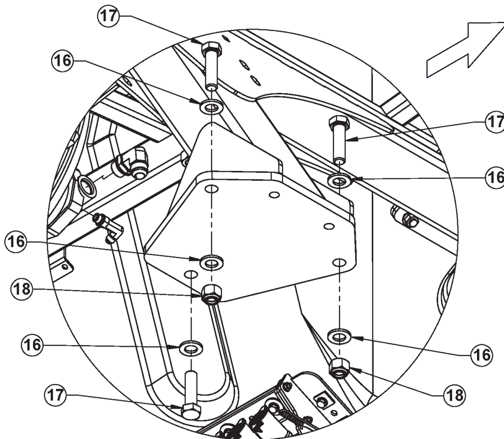
DETAIL B SCALE 1 : 6
