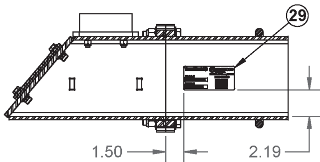
Secondary Serial Number Decal Installation
