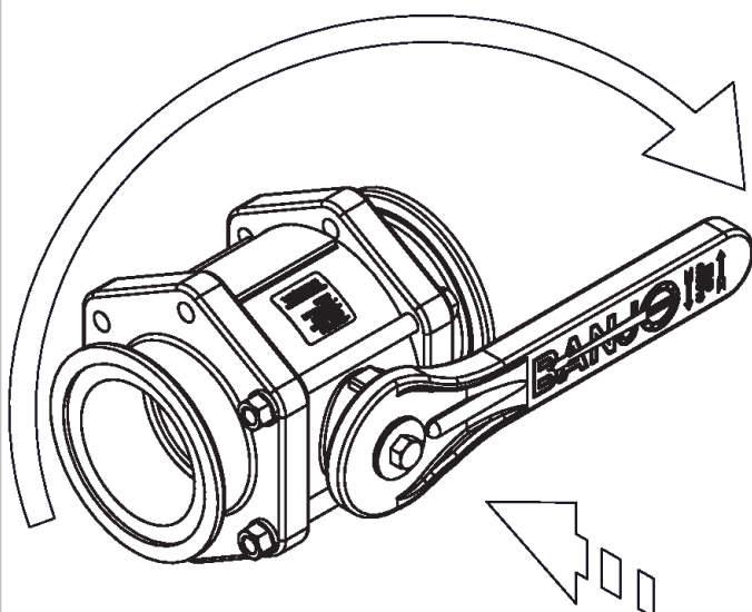
3. Flip handle 180° and re-install 3/8" bolt and washer. With the handle correctly installed, the handle will be orientated as shown in the open position.
