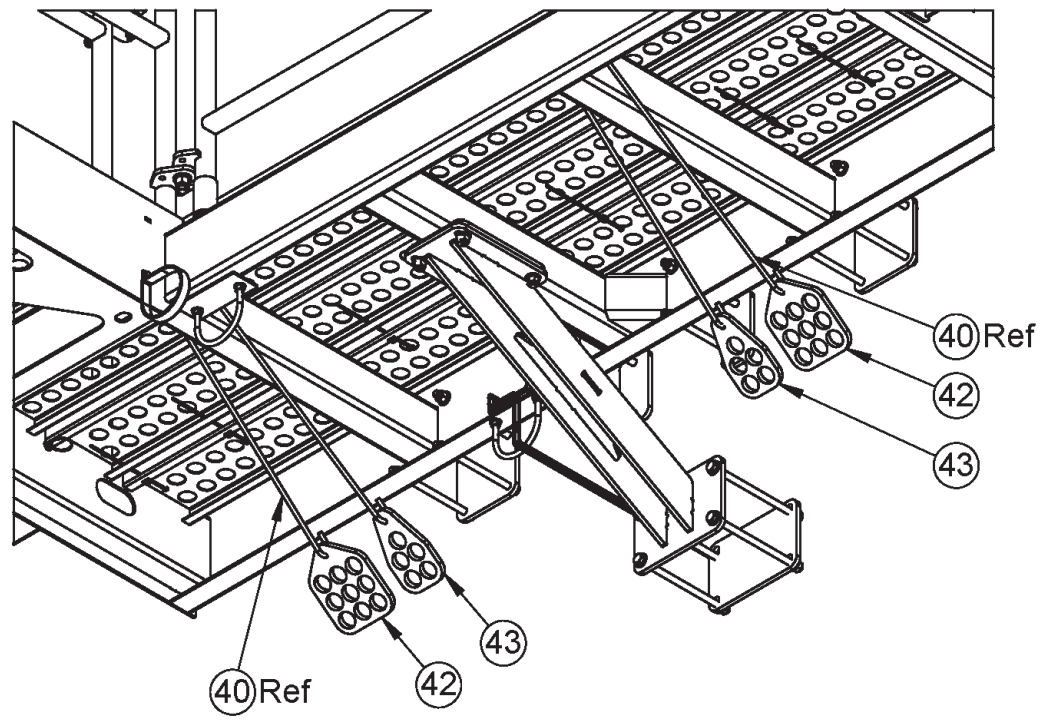
J-Hangers
