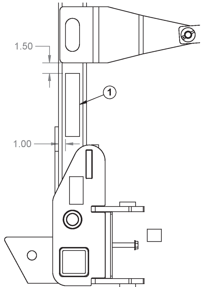
Rear View Left Wing Row Marker Decal Locations (Repeat for Right Wing)
