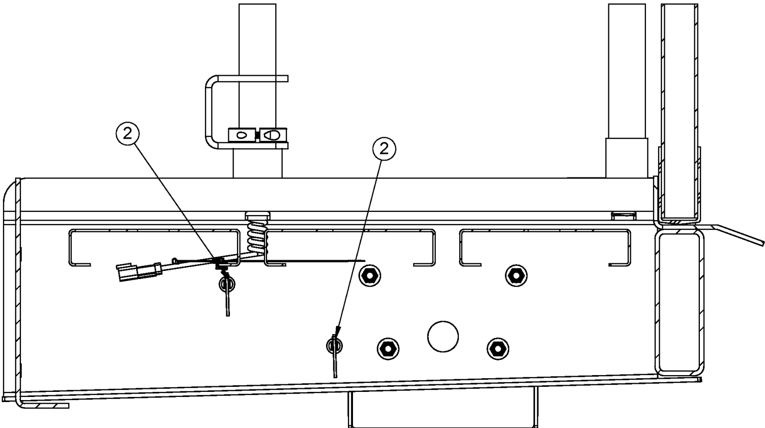
Cable Tie Mount Locations (Right Side, Looking Outward)
