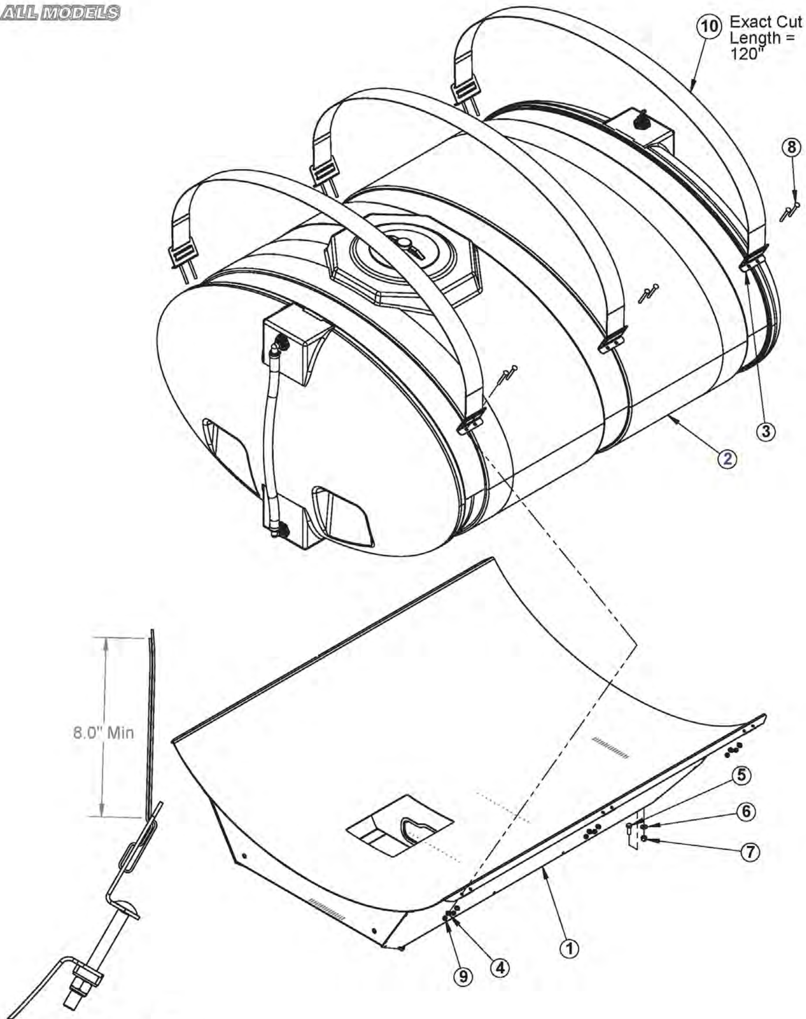
Webbing Routing Detail
