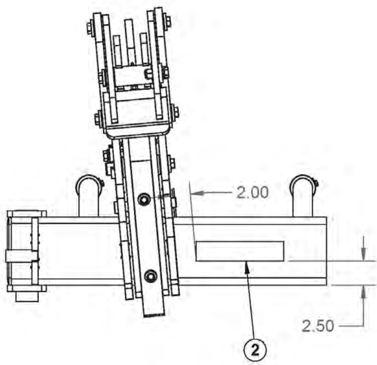
Looking towards back of machine from end row unit
