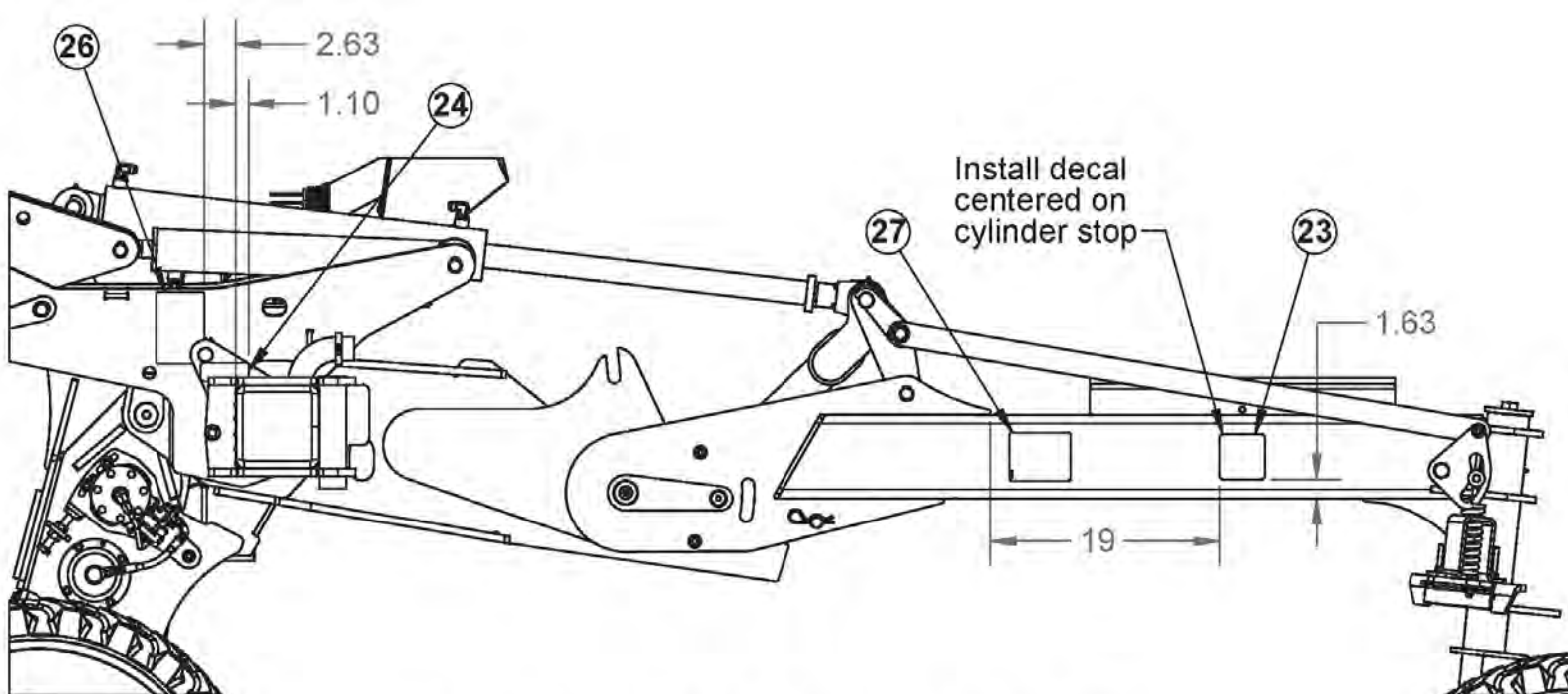
Looking towards center of machine from left end
