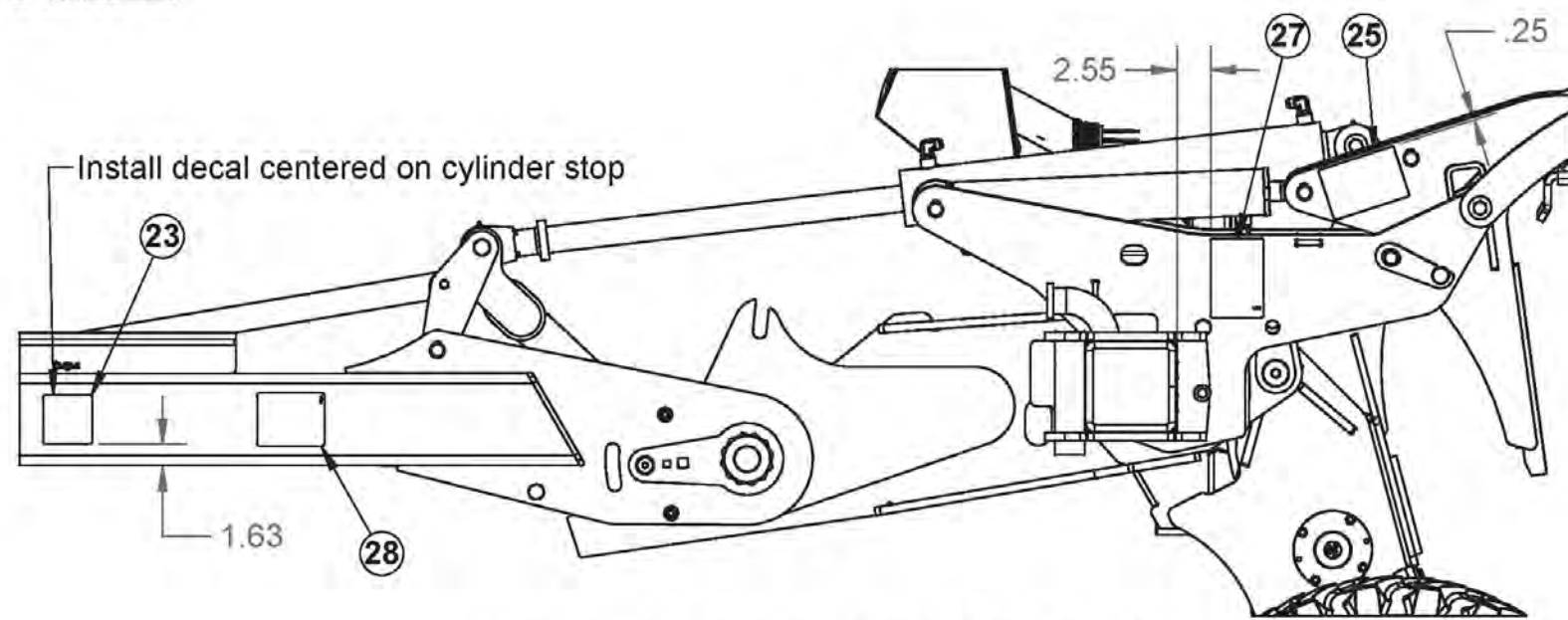
Looking towards center of machine from right end
