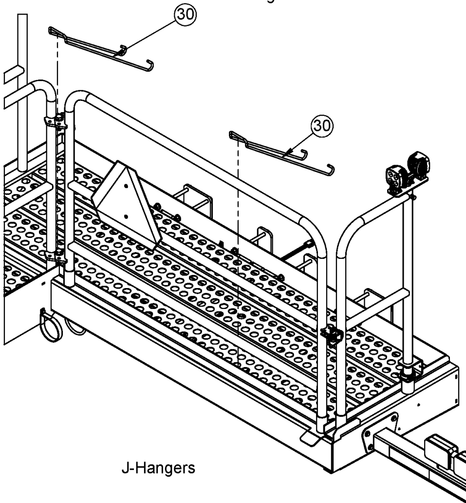
J-Hangers
