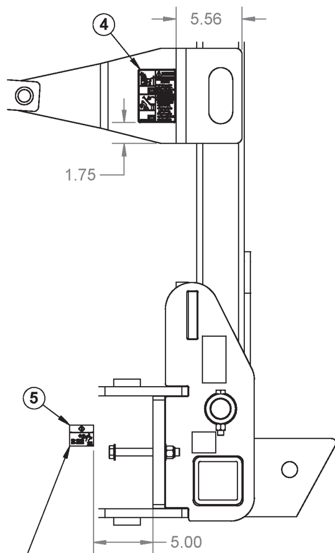
Front View Left Wing Row Marker Decal Locations (Repeat for Right Wing)
