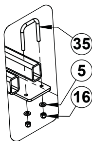
DETAIL J SCALE 1 : 15
