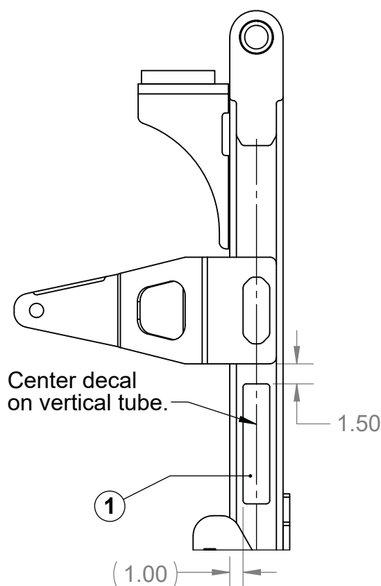
Back View Yellow Reflector Installation
