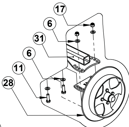
DETAIL E SCALE 1 : 15
