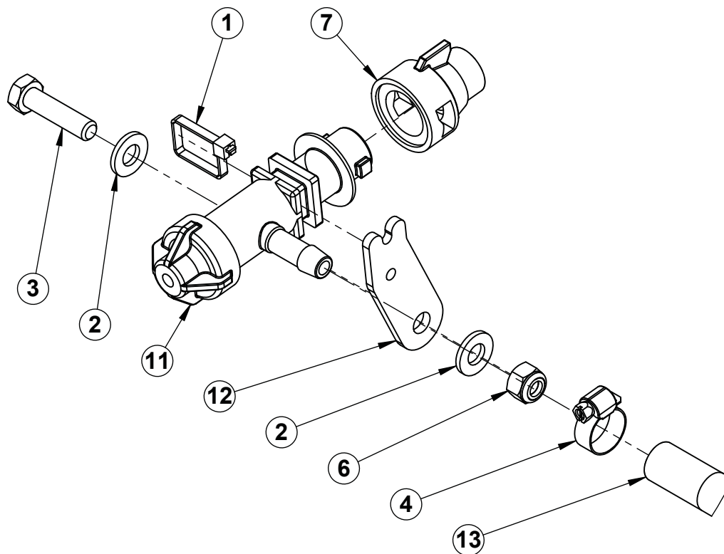
DETAIL C SCALE 1 : 2
