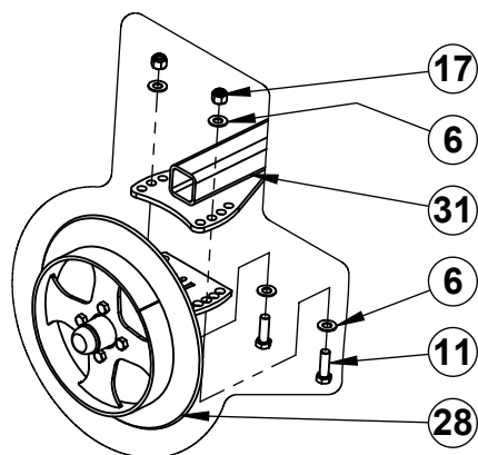
DETAIL A SCALE 1 : 15
