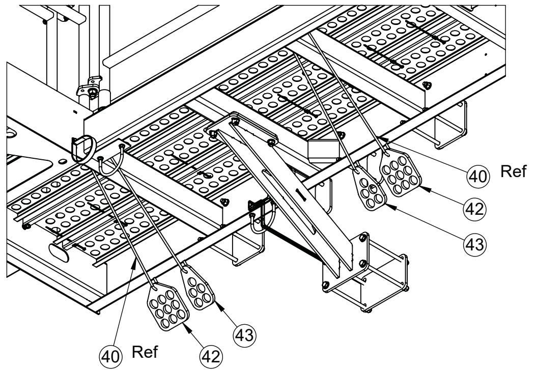
J-Hangers
