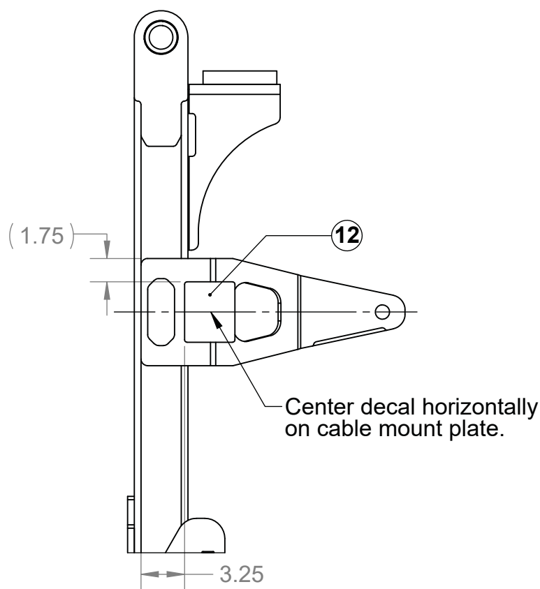
Front View Danger-Warn Decal Installation
