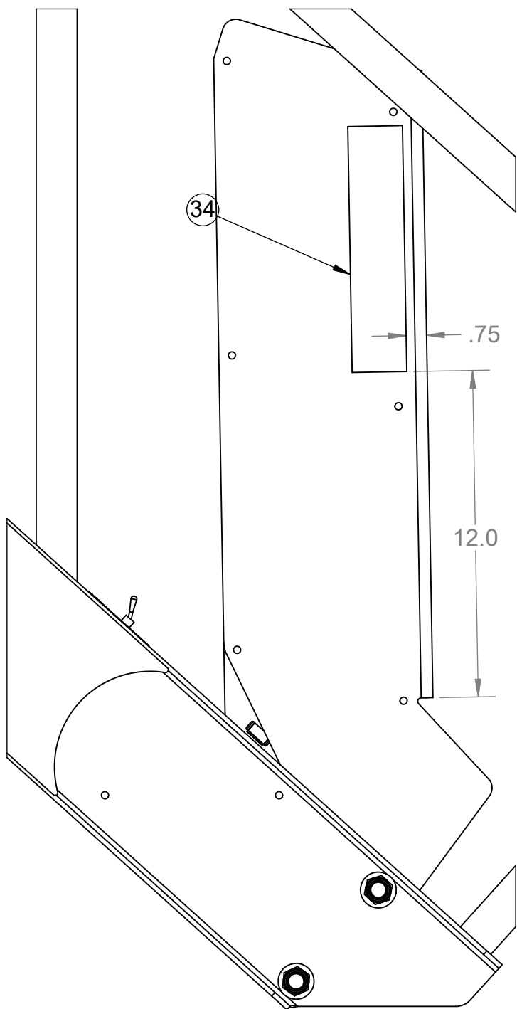
Left Hand Ladder View
