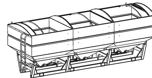
Model 900 • 8ft by 24ft box, 3 compartments, 900 Cubic feet (Struck), 304 Stainless Steel, Vibrator mounts between compartments.
