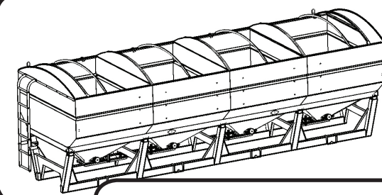
Model 785 • 8ft by 24ft box, 4 compartments, 785 Cubic feet (Struck), 304 Stainless Steel, Vibrator mounts between compartments.
